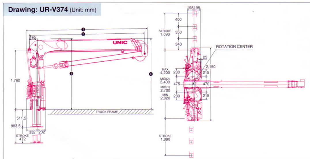
Crane Mounting Dimensions
